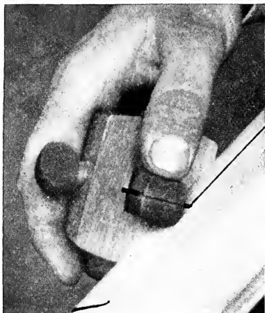
Fig. 51—Rolled Gauge
